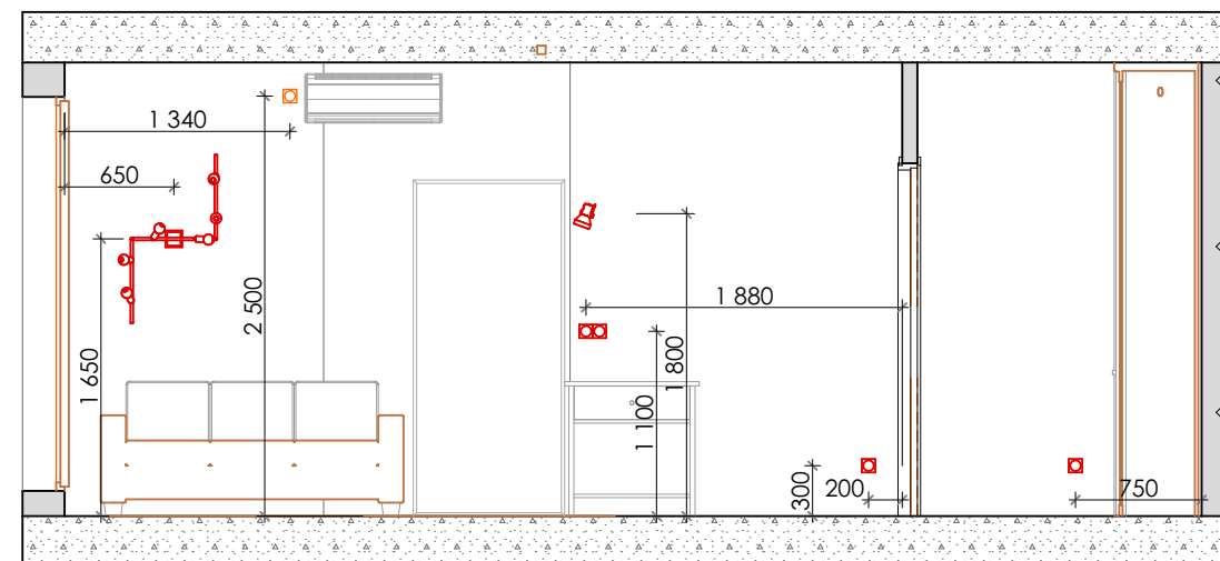
S-02 Building Section 1:50
