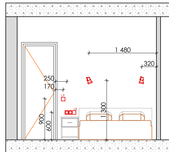
S-01 Building Section 1:50
