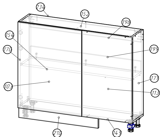
1_Низ_1118_232_914
