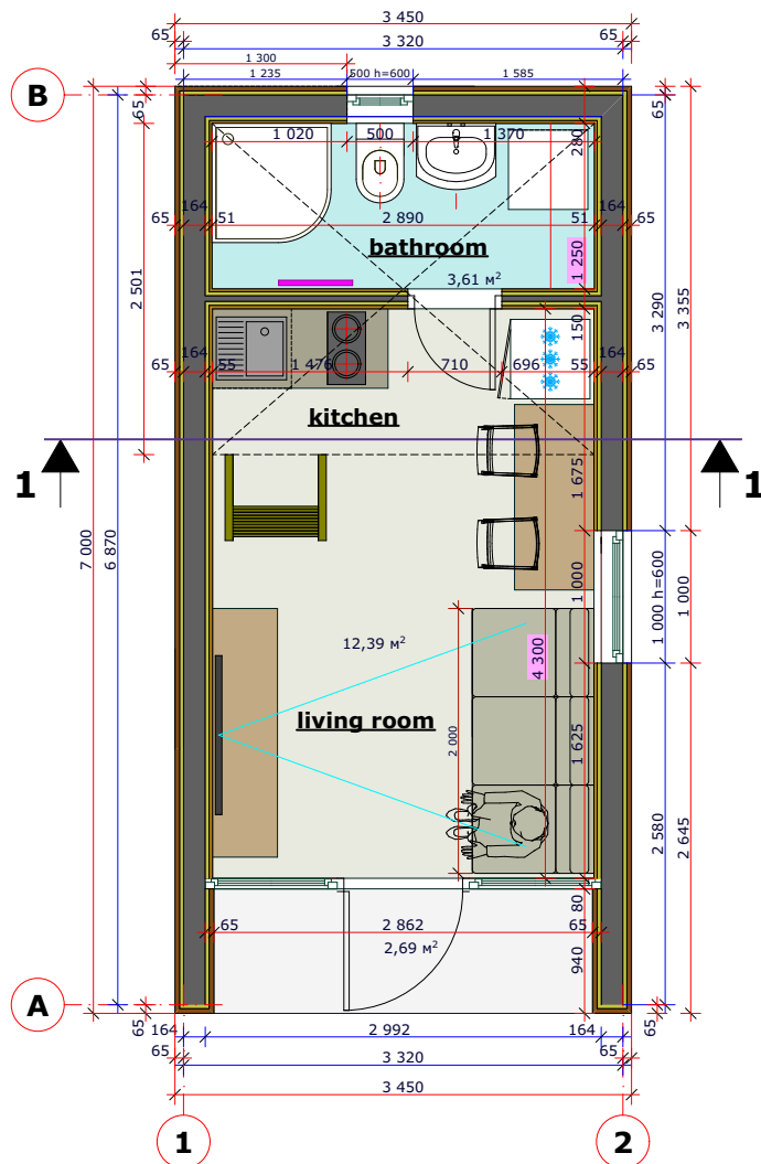
House plan 1
