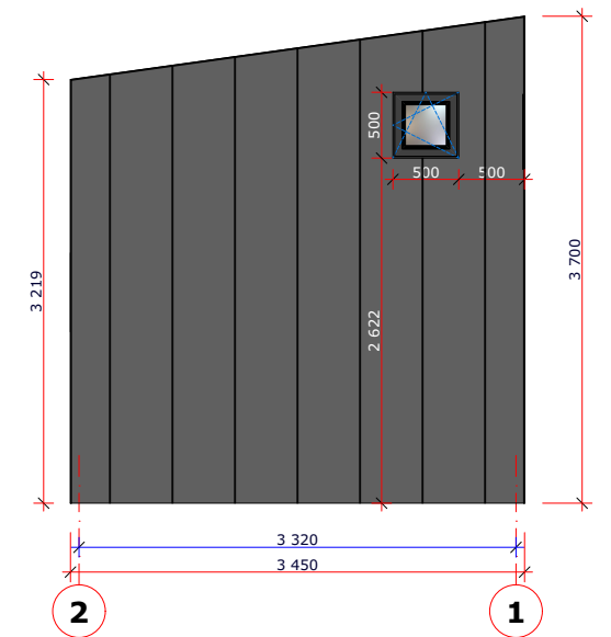
Facade 2 - 1
