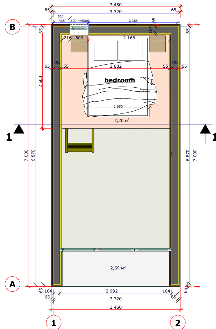
House plan 2
